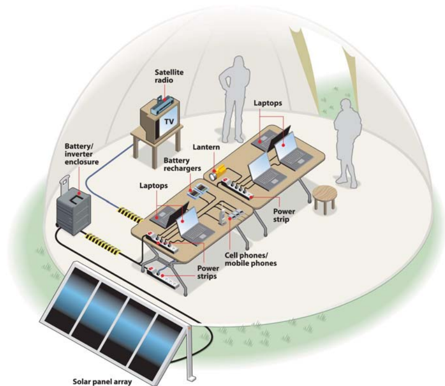
ABOVE: The 200W solar array deployed outside a Shelter Systems emergency dome-shelter. BELOW: Shows the typical “inside-the-dome-shelter” setup for powering a wide range of devices.
