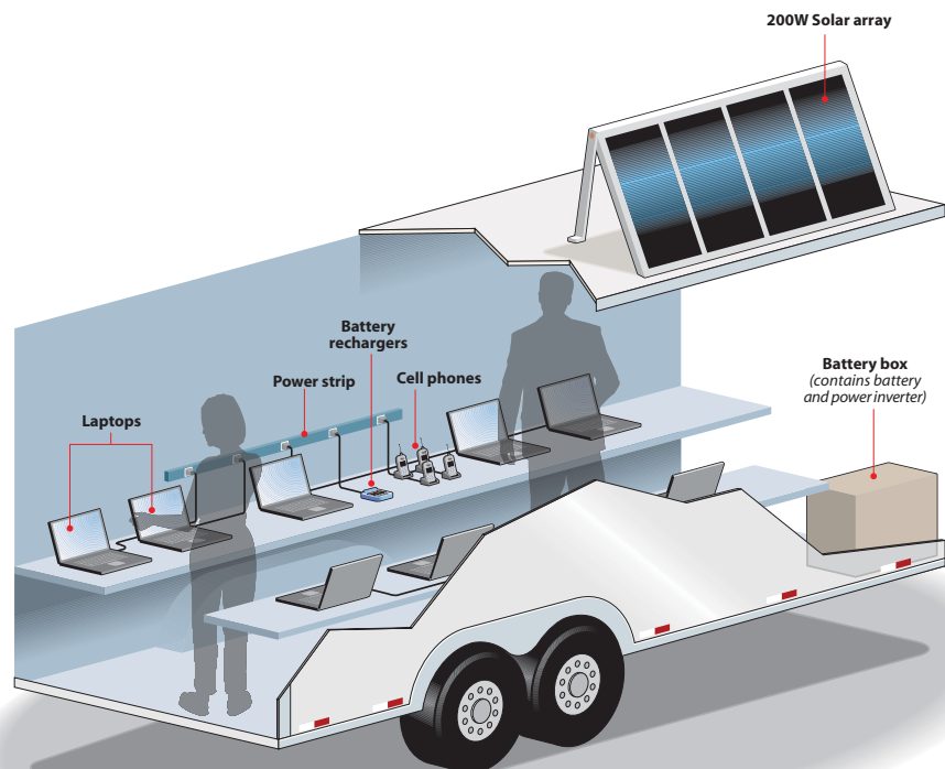
BELOW: Shows the typical "inside-the-trailer" setup for powering a wide range of devices.
